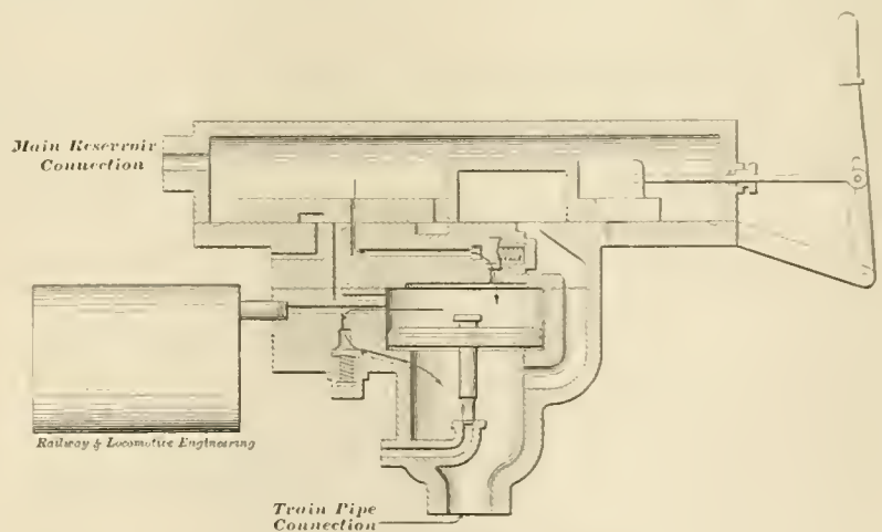
A NEWLY PATENTED BRAKE VALVE—RUNNING POSITION
